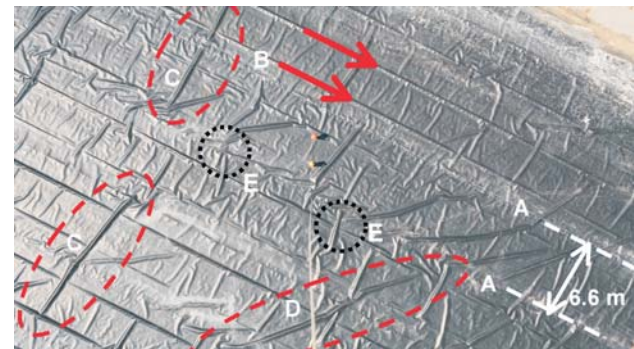
Figure 7 - Air photo of geomembrane installation. 1.5 mm smooth HDPE; Camera elevation 65 m; Latitude 43 \text{ }^\circ 16' \text{ N} ; Air temperature 28 \text{ }^\circ\text{C} ; 1:20 pm Aug 18 2006 (modified from Chappel et al. 2007).
