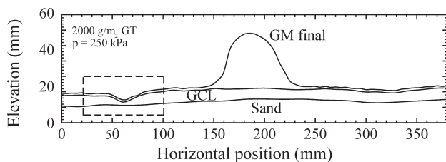
Figure 10 - Cross-section through Fig. 9 at the location of minimum GCL thickness (adapted from Dickinson & Brachman, 2006).
