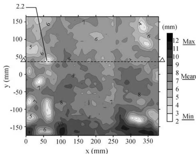
Figure 9 - Contours of the final thickness of a GCL after application of 250 kPa vertical pressure. Configuration comprised (from top down) nominal 50 mm gravel, for a 2000 \text{ g/m}^2 needle-punched nonwoven protection layer, geomembrane and GCL ( w = 115\% ), sand layer (adapted from Dickinson & Brachman, 2006). Marked cross-section shown in Fig. 10.
