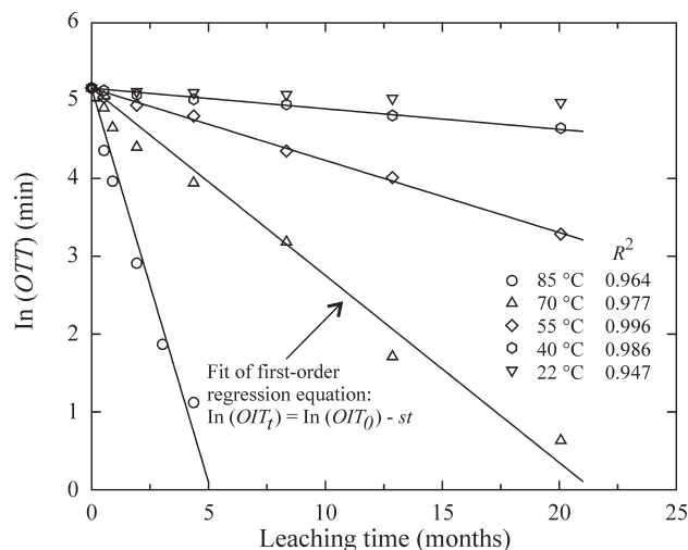
Figure 15 - Variation in \ln(\text{OIT}) with time at different temperatures in leachate. \text{OIT}_o is the initial OIT and \text{OIT}_t is the OIT at time t (month), s is the antioxidant depletion rate ( \text{month}^{-1} ) (after Islam & Rowe, 2007).
