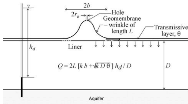
Figure 11 - Schematic defining leakage through a composite liner with a wrinkle. Assumes lateral migration at interface and vertical flow in clay liner.
