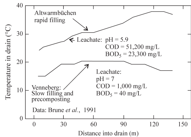
Figure 3 - Temperature in drains at two German landfills approximately 4 years after last waste placed above the drains (modified from Brune et al. , 1991).
