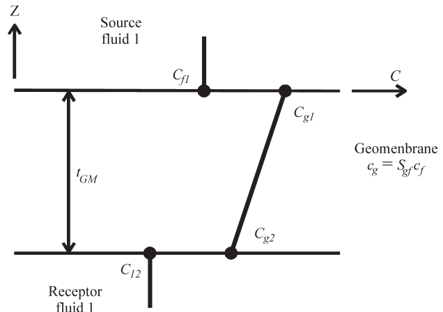
Figure 14 - Concentration profile for diffusion across a geomembrane showing (a) partitioning between the concentration in the source solution, c_{f1} , and the concentration in the adjacent geomembrane, c_{g1} ; (b) diffusion profile from the top to bottom of the geomembrane; (c) partitioning between the concentration at the bottom of the geomembrane, c_{g2} and the concentration in the receptor solution, c_{f2} . Note that c_{g1}/c_{f1} = c_{g2}/c_{f2} = S_{gf} .
