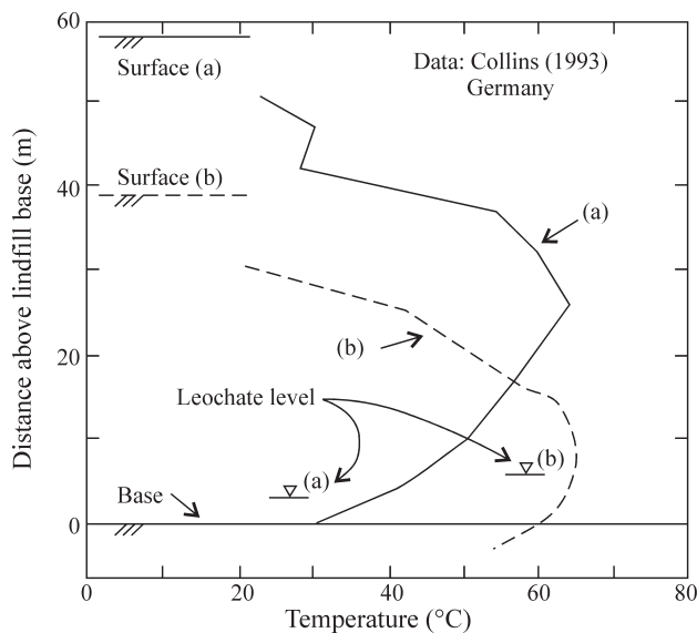
Figure 2 - Temperature variation with depth at two locations, (a) and (b), in an old landfill (1936-1980) in Hannover Germany; waste circa 1938 at bottom (after Rowe, 1998).
