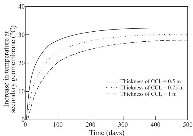
Figure 5 - Effect of primary liner thickness on temperature of secondary geomembrane assuming a 40 °C increase on the primary liner (after Rowe & Hoor, 2007).
