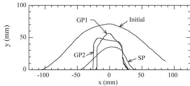
Figure 8 - Wrinkle geometry in a 1.5 mm HDPE geomembrane before and after application of 1000 kPa vertical pressure for 10 h. Results shown for sand above and below the geomembrane (SP) and 50 mm gravel directly above and a GCL beneath the geomembrane at two locations on the wrinkle: GP1 and GP2 (after Rowe et al. 2004b).
