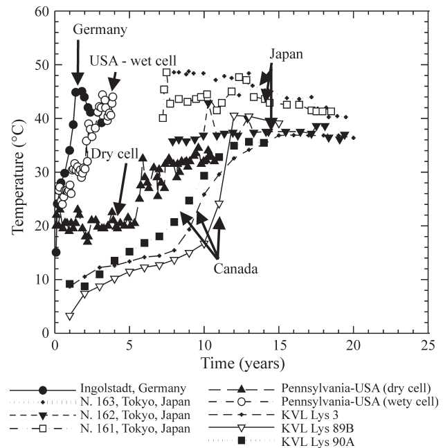
Figure 4 - Some observed temperatures at the base of landfills (US data: Koerner & Koerner, 2006; Canadian data: Rowe, 2005; Japanese data: Yoshida & Rowe, 2003; German data: Klein et al. 2001).
