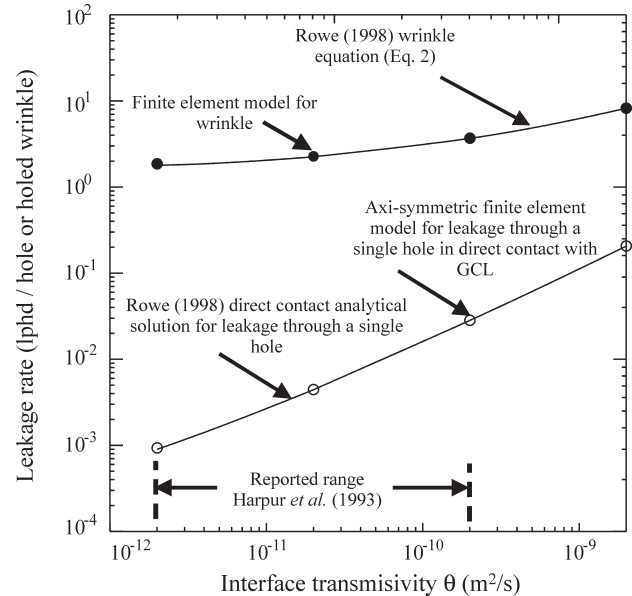
Figure 12 - Comparison of leakage rates for GM/GCL/attenuation layer composite liner and a range of interface transmissivities as calculated from analytical solutions and FEM analysis for (a) a single hole in direct contact with the GCL and (b) a single 15 m long wrinkle with a hole. k_L = 5 \times 10^{-11} m/s, H_L = 0.01 m, k_f = 1 \times 10^{-6} m/s, H_f = 0.5 m, L = 15 m, B = 30 m and 2b = 0.3 m.
