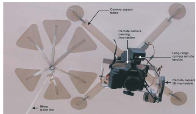
Figure 6 - Photograph showing digital camera mounted to the underside of the blimp (after Chappel et al. 2007).
