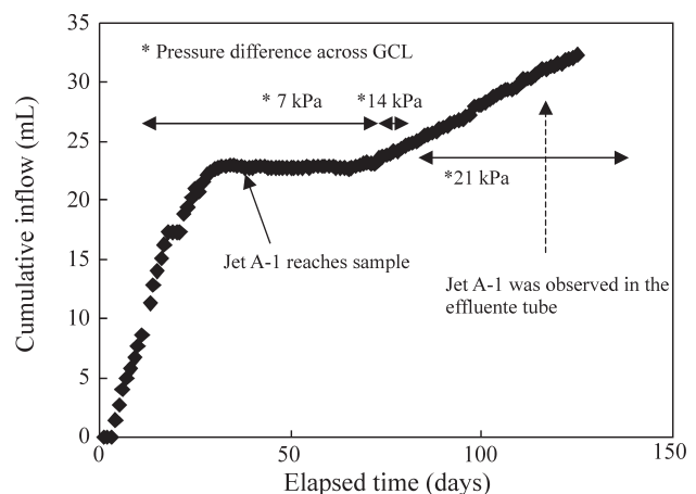
Figure 1 - Variation in cumulative inflow volume through the GCL with time for a GCL subjected to 12 freeze and thaw cycles and permeated with water and Jet A-1 in flexible wall permeameter test (modified from Rowe et al. , 2005c).
