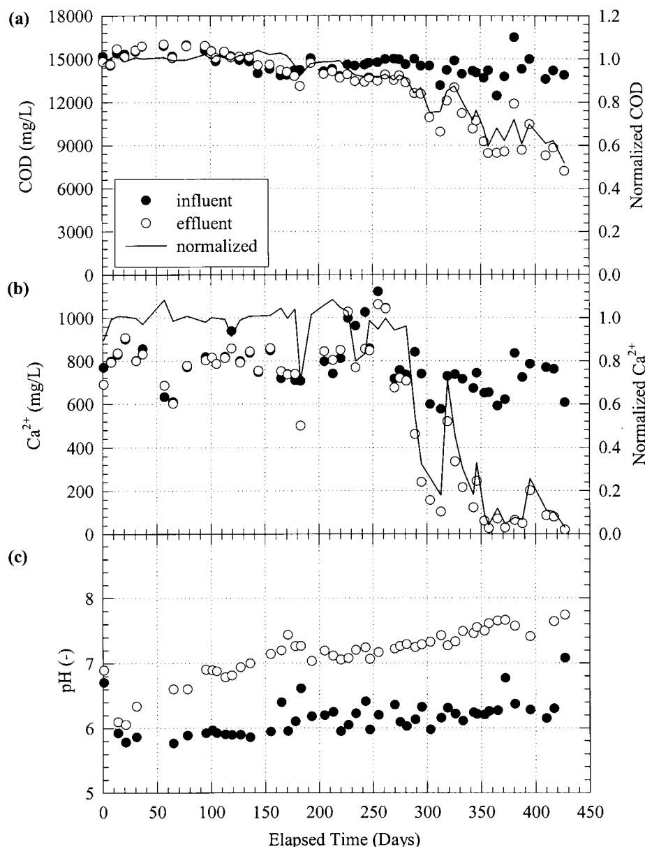
Figure 2. Variation in influent and effluent synthetic leachate characteristics with time: (a) COD (measured) versus elapsed time, (b) Ca 2+ versus elapsed time, and (c) pH versus elapsed time.
