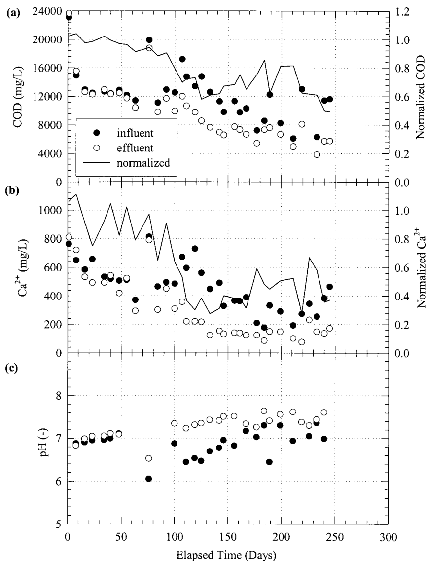
Figure 3. Variation in influent and effluent KVL leachate characteristics with time: (a) COD (measured) versus elapsed time, (b) Ca 2+ versus elapsed time, and (c) pH versus elapsed time.
