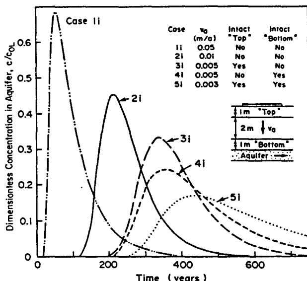
FIG. 4. Variation in chloride concentration in the aquifer, assuming migration along fractures.
