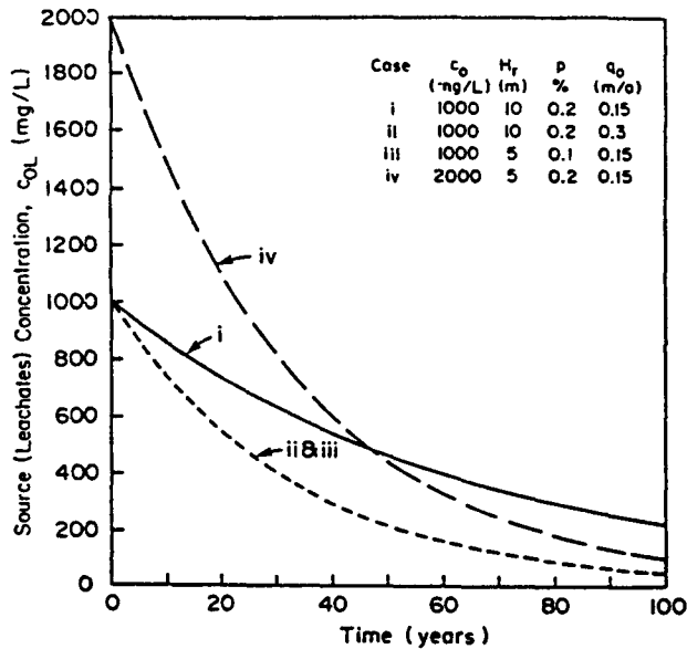
FIG. 1. Decrease in leachate (chloride) concentration with time.
