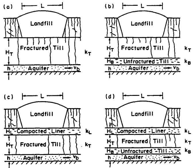
FIG. 2. Cases considered: (a) cases 0, 1, and 2; (b) case 4; (c) case 3; (d) case 5.
