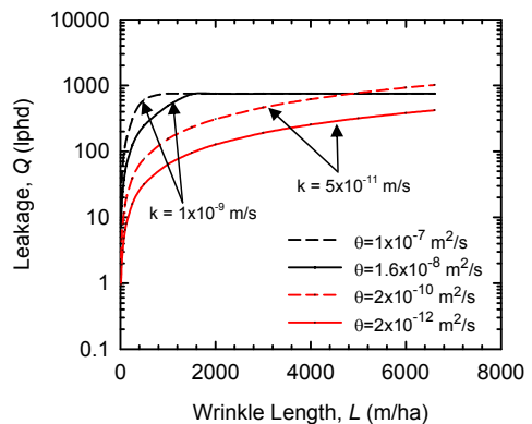
Figure 6. Leakage through a hole in an interconnected wrinkle of length L (in metres per hectare) for a single composite liner with (i) CCL with k=1 \times 10^{-9} m/s and “poor” contact away from wrinkles, \theta=1 \times 10^{-7} m 2 /s, (ii) CCL with k=1 \times 10^{-9} m/s and “good” contact away from wrinkles, \theta=1.6 \times 10^{-8} m 2 /s, (iii) GCL with k=5 \times 10^{-11} m/s and “poor” contact away from wrinkles, \theta=2 \times 10^{-10} m 2 /s, and (iv) GCL with k=5 \times 10^{-11} m/s and “good” contact away from wrinkles, \theta=2 \times 10^{-12} m 2 /s.
