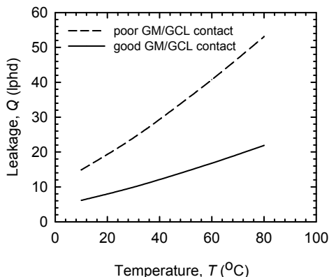
Figure 9. Effect of temperature on leakage through a hole in a 125m/ha wrinkle in a GM over a GCL for “good” and “poor” contact conditions (Base case parameters at 20°C: k=5 \times 10^{-11} m/s and “good” \theta=2 \times 10^{-12} m 2 /s, “poor”, \theta=2 \times 10^{-10} m 2 /s)
