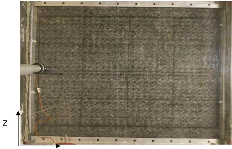
Figure 5: Installation of GCL in the big-box model
