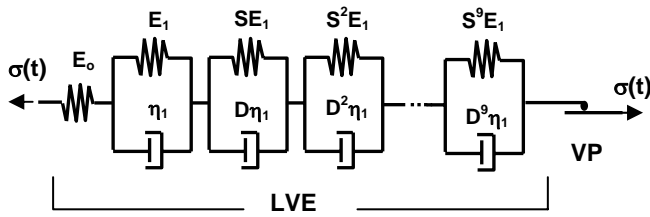
Figure 2: The LVE-VP model
